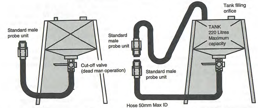
3B: Overhead rig with return vent and refuelling hose
