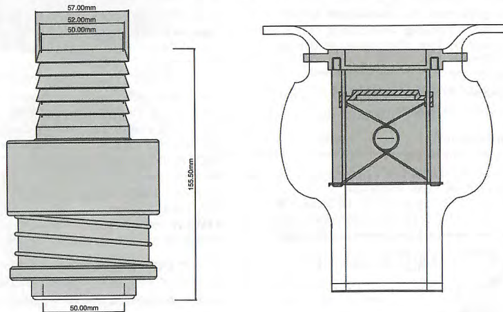
Diagram 1: General Design of Dry Break Coupling
