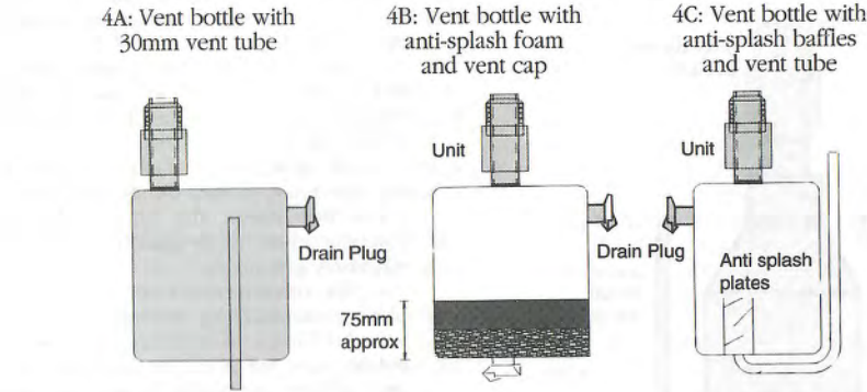
Diagram 4: General Design of Vent Bottles
