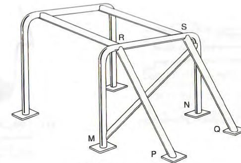
Type 5 Full Cage
