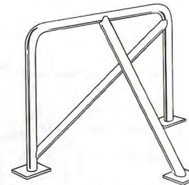
Type 3 Full Width Braced Roll Bar
