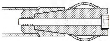
Fig 5 Tapered Connection
