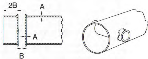
Fig 3 Sleeving a Hoop or Brace
